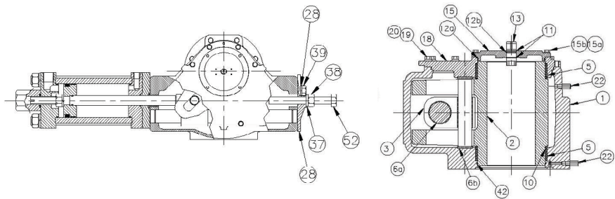
HP65 and HP80 Series Yoke shown at mid-stroke pointer omitted for clarity
