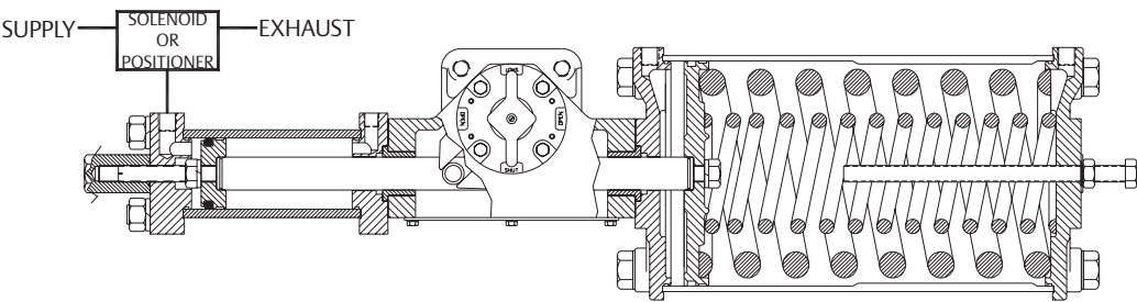
Figure 1 Single Acting, Two Cylinders
