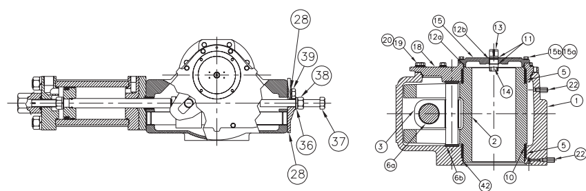
HP65 and HP80 Series Yoke shown at mid-stroke pointer omitted for clarity
