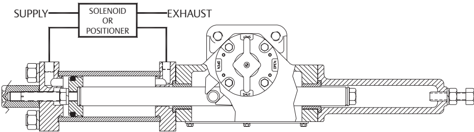
Figure 3 Double-Acting, Single Cylinder
